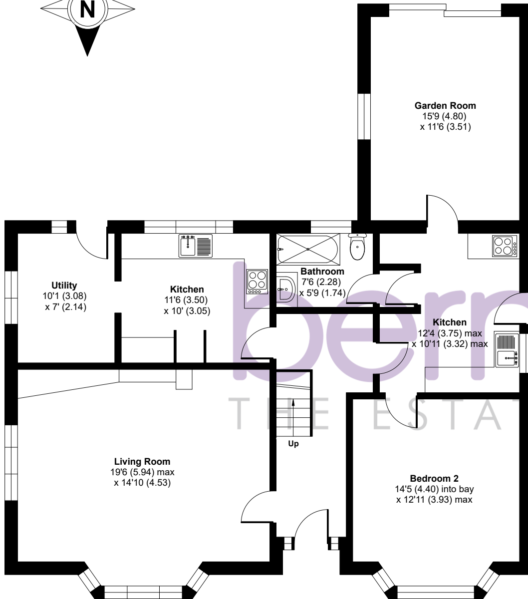
GROUND FLOOR
